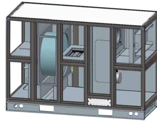
Rotary recovery system with damper for air recirculation
