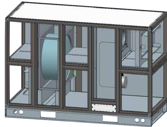
Rotary recovery system with 100% exterior air
