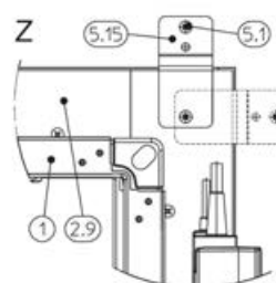
Fig. 17: Installation kit – clear space, normal installation
