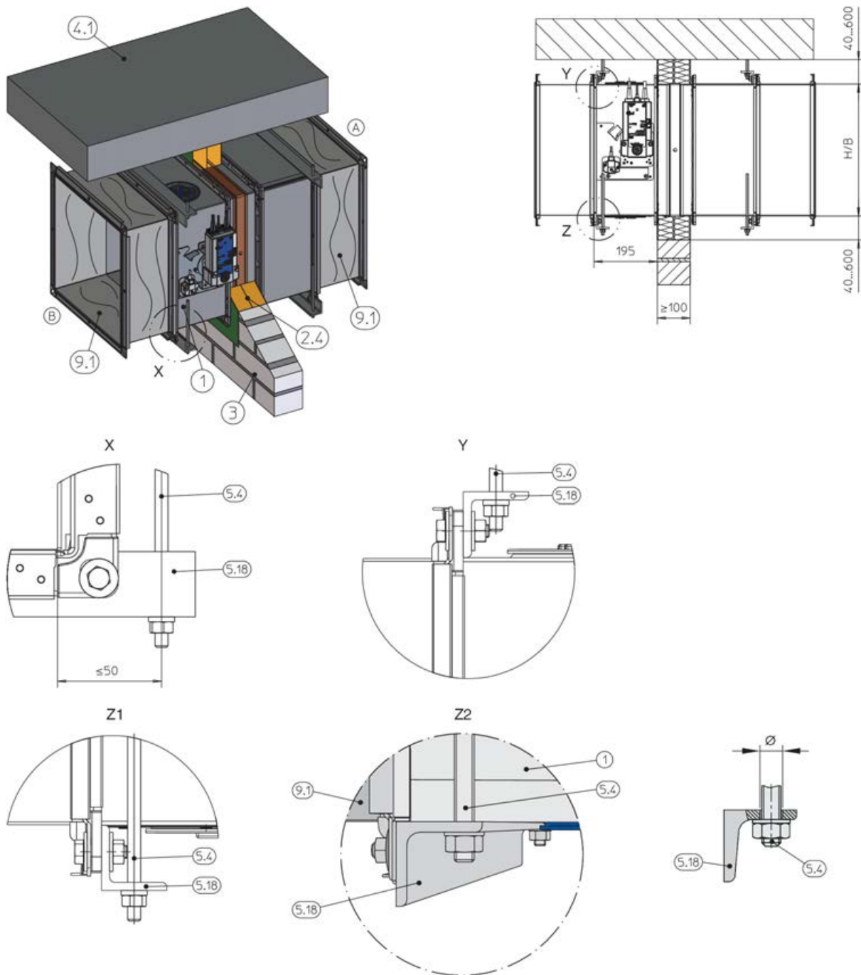
Fig. 40: Fixing of FK2-EU, wall installation with a fire batt
