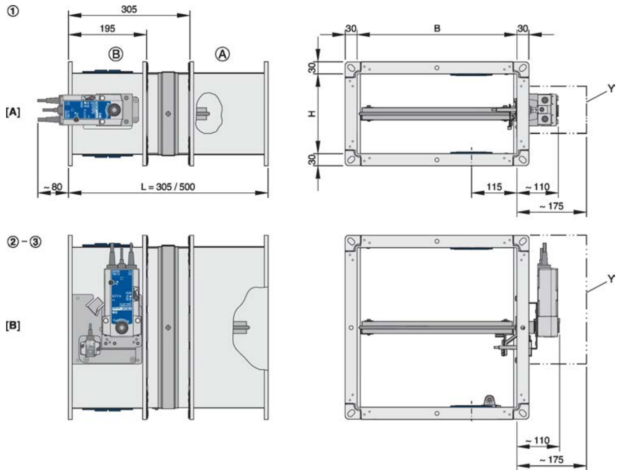
Fig. 5: FK2-EU with Belimo spring return actuator
