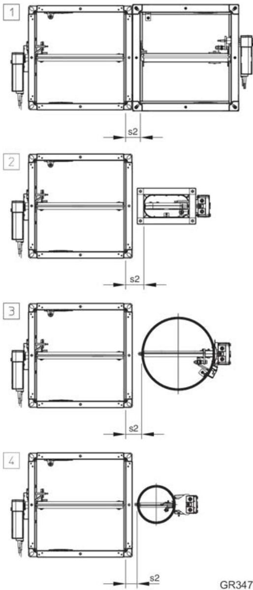
Fig. 22: Distance between FK2-EU and other TROX fire dampers in mortar-based installation
