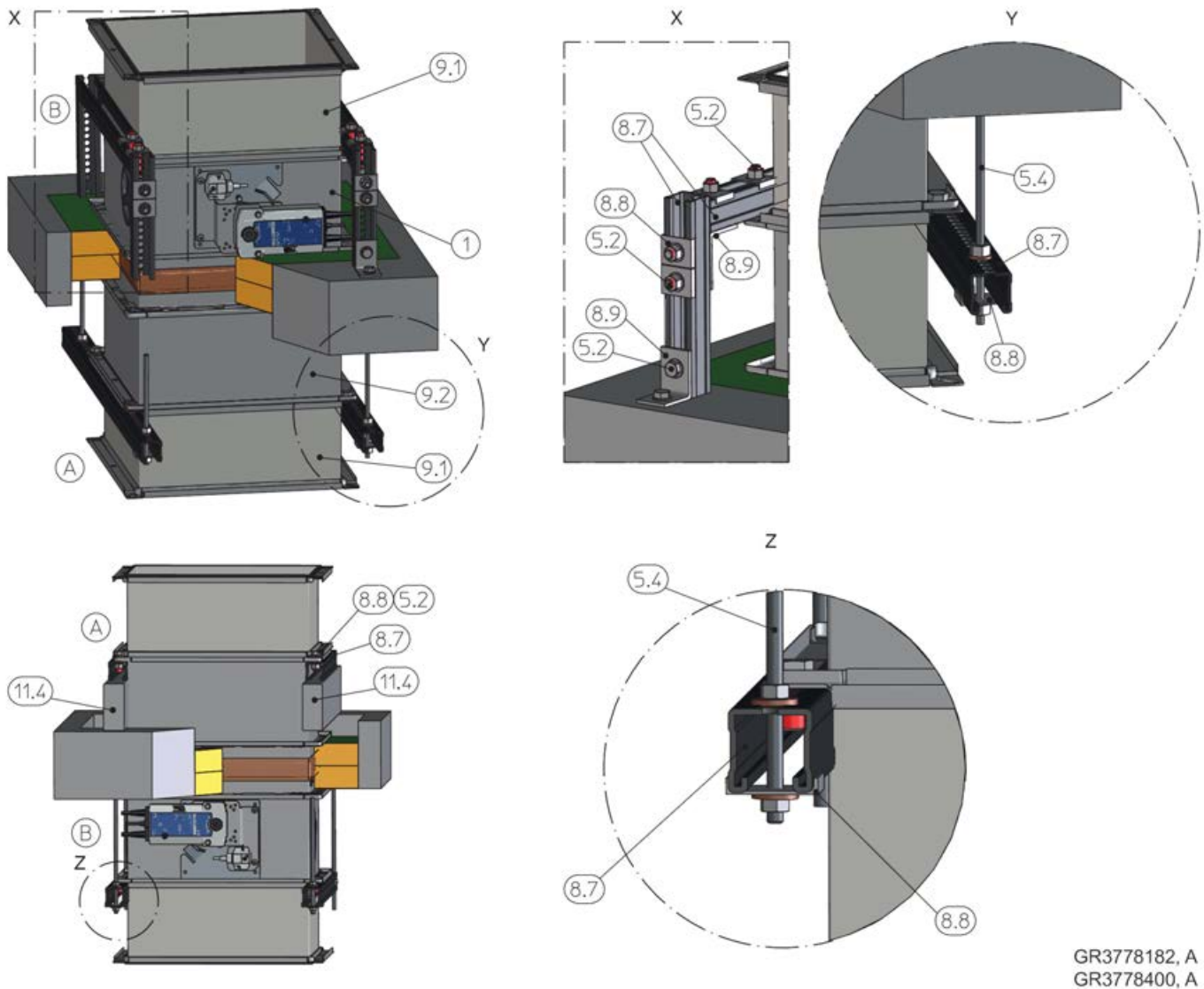
Fig. 41: Suspension in fire batt, FK2-EU upright or suspended
