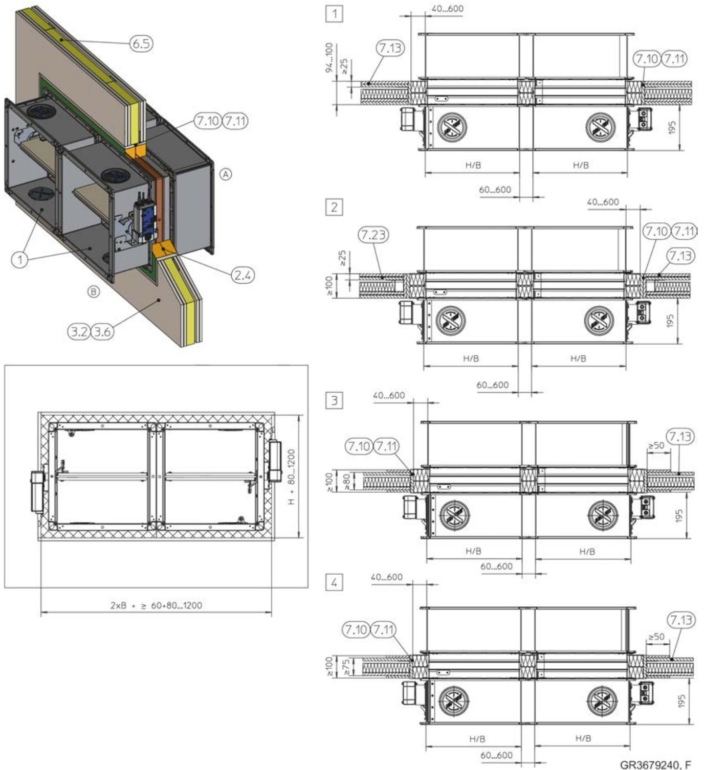
Fig. 37: Dry mortarless installation into a lightweight partition wall, with a fire batt, flange to flange, illustration shows side by side installation (applies also to installation of dampers on top of each other)
