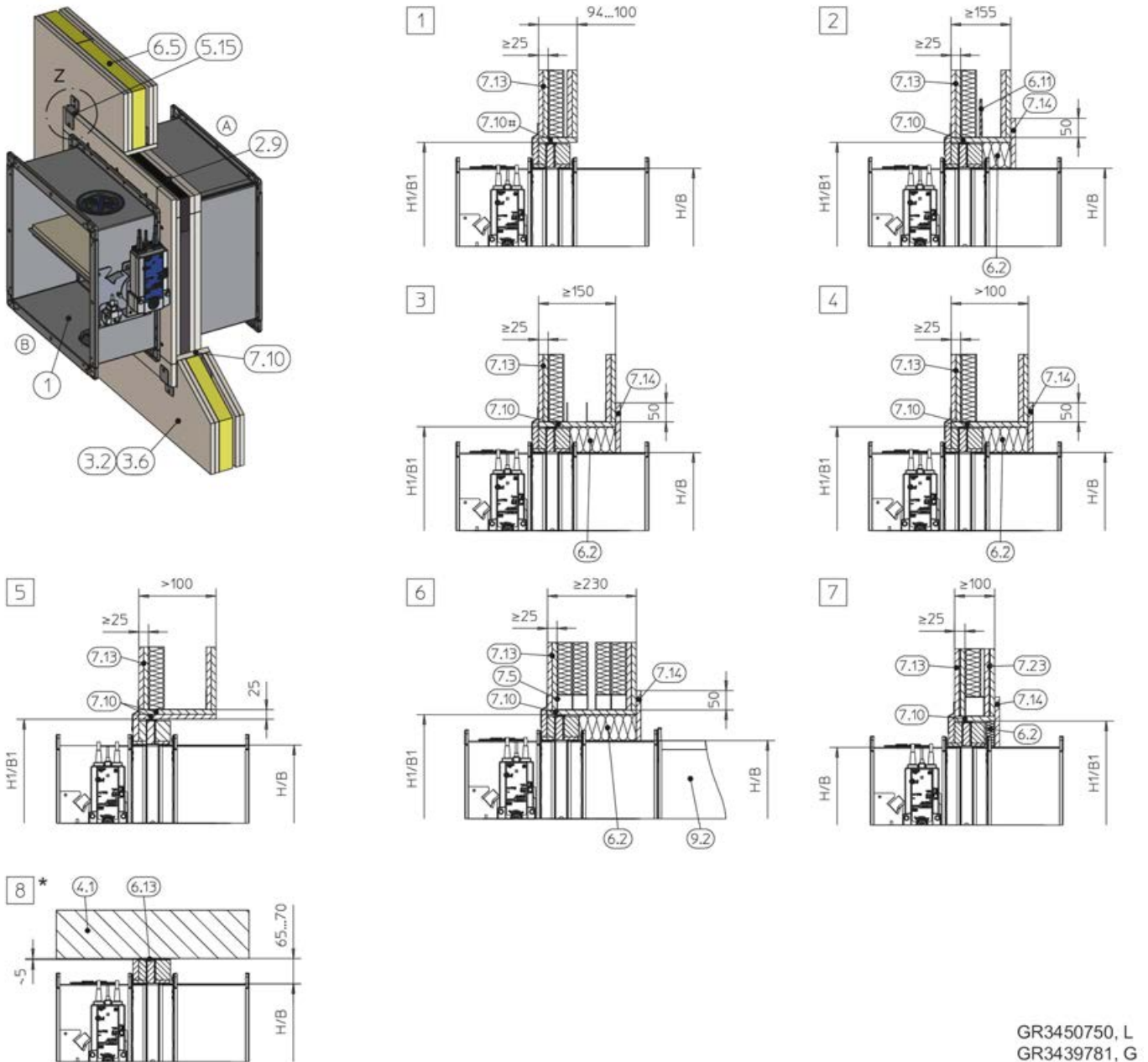
Fig. 32: Dry mortarless installation into a lightweight partition wall, with installation kit ES
