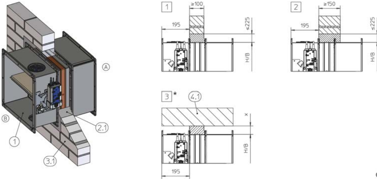
Fig. 24: Mortar-based installation into a solid wall
