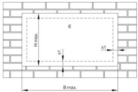
Fig. 21: Fire batt – installation in solid walls and ceiling slabs, lightweight partition, timber stud wall, half-timbered construction and solid wood walls
