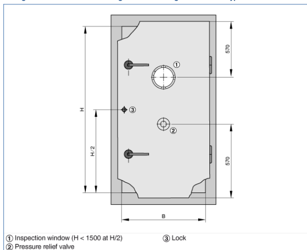
Arrangement of attachments for single leaf low-leakage steel door of Type ST
