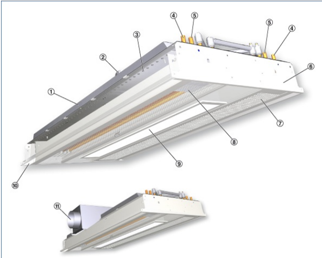
Schematic illustration of DID600B-L
